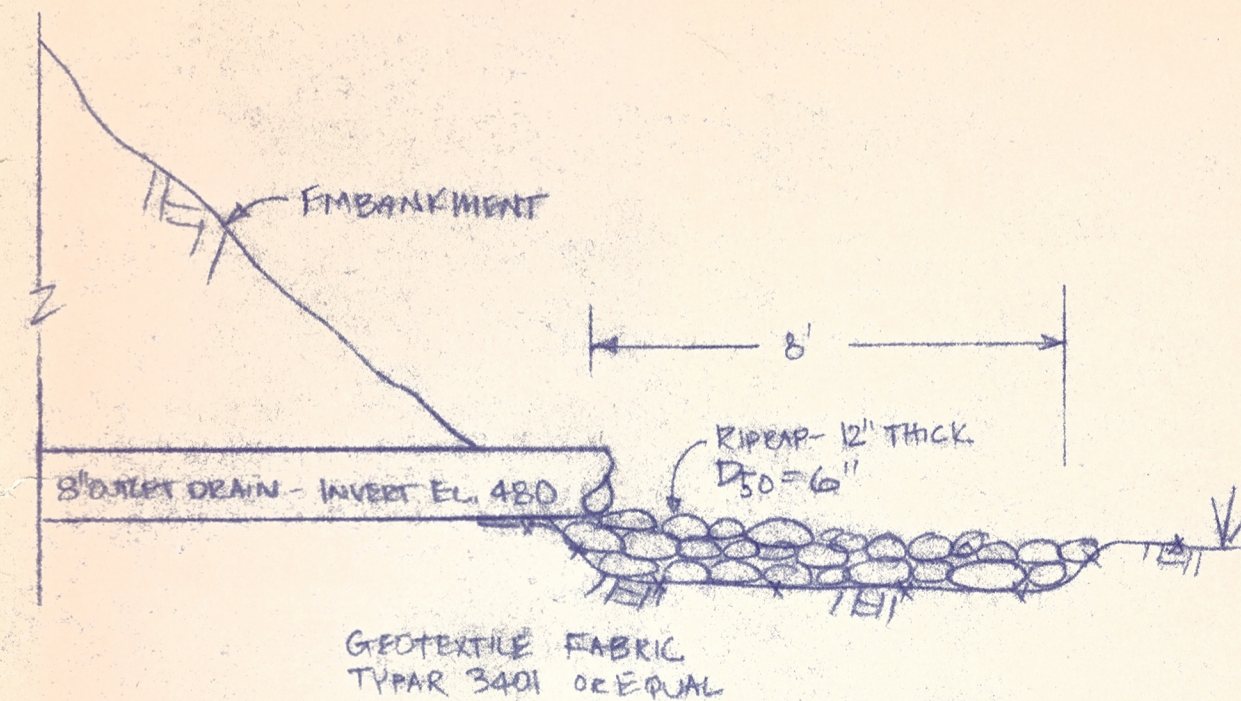
DRAIN OUTLET NOT TO SCALE
