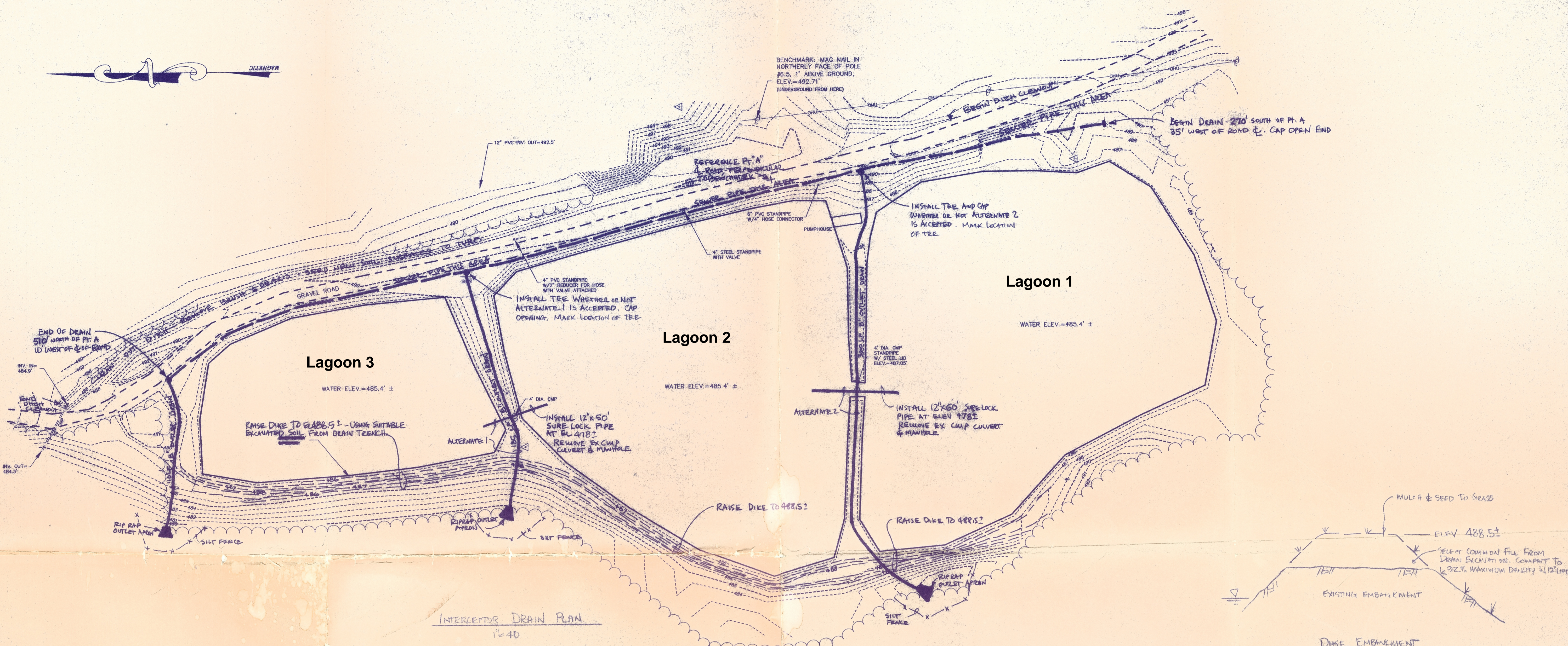
DIKE EMBANKMENT NTS
