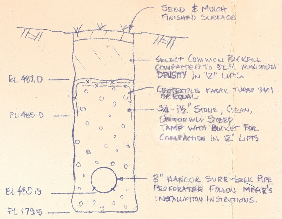
DRAIN TRENCH NOT TO SCALE
