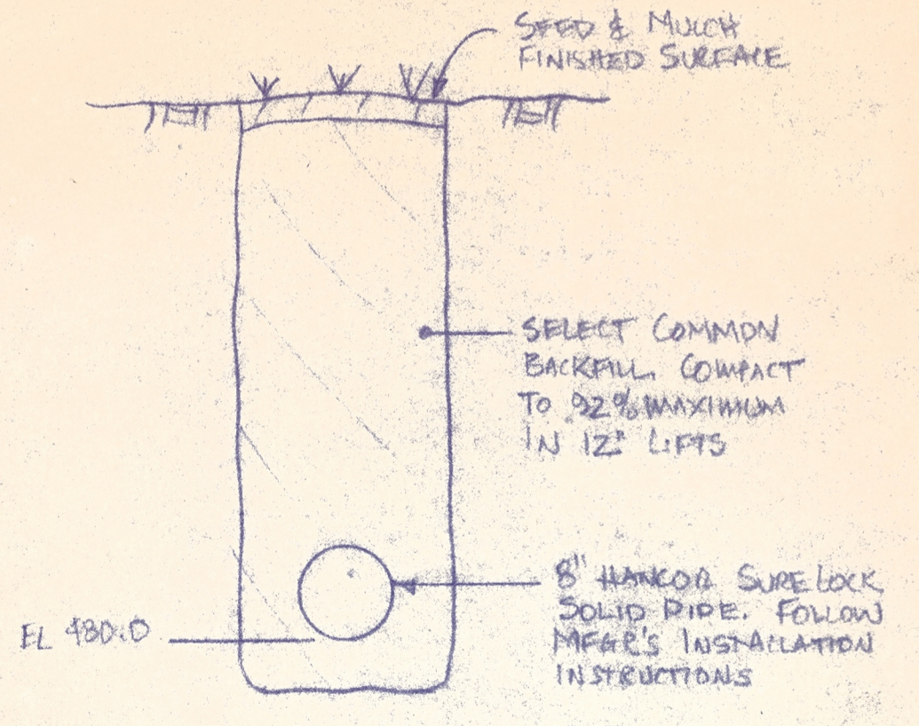
OUTLET TRENCH NOT TO SCALE
