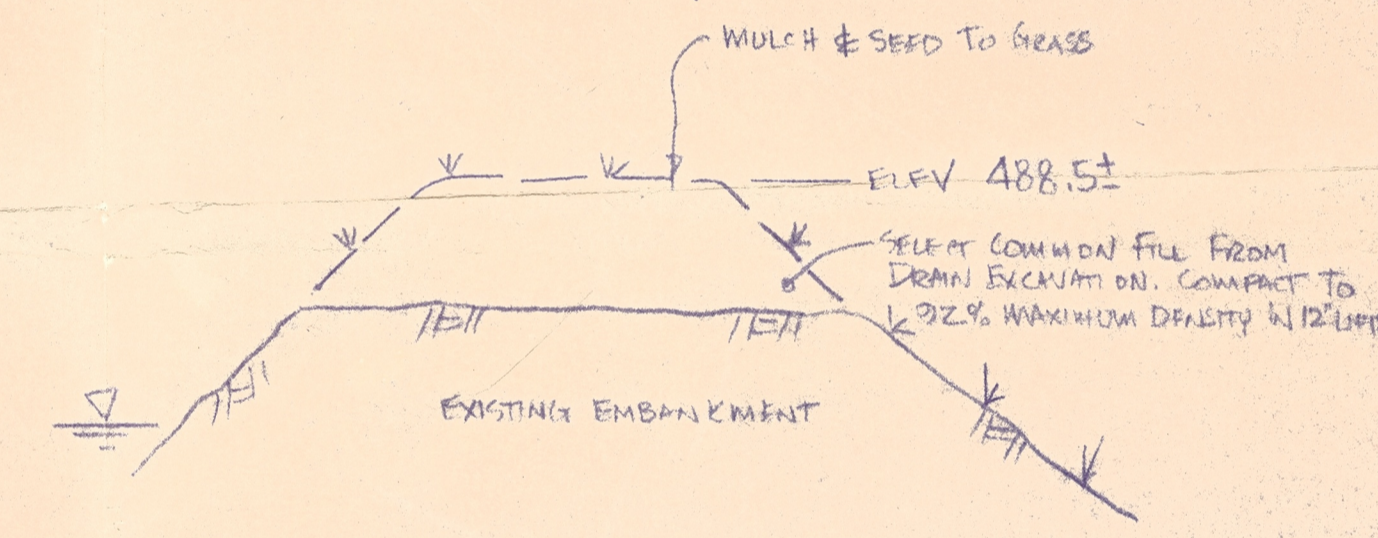
DIKE EMBANKMENT NTS
